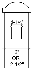
BEFREE™ WALL POST DETAIL SCALE: 3" = 1'-0"
