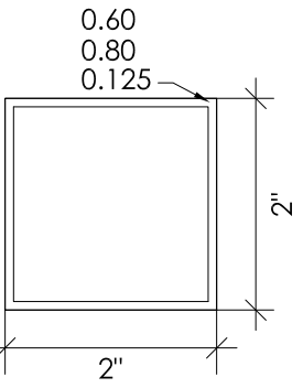
WALL POST TOP VIEW SCALE: 6" = 1'-0"
