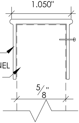
PICKET FASTENED TO CHANNEL DETAIL SCALE: 1" = 1'-0"
